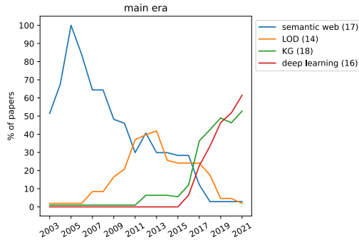
Fig. 7. Timeline for the percentages of main papers from each year that match the sub-themes Semantic Web, LOD, KGs, and deep learning. 8
